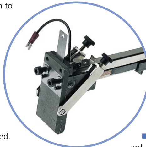
The NAGEL stapling head.
